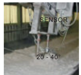
Aluminium oxide
